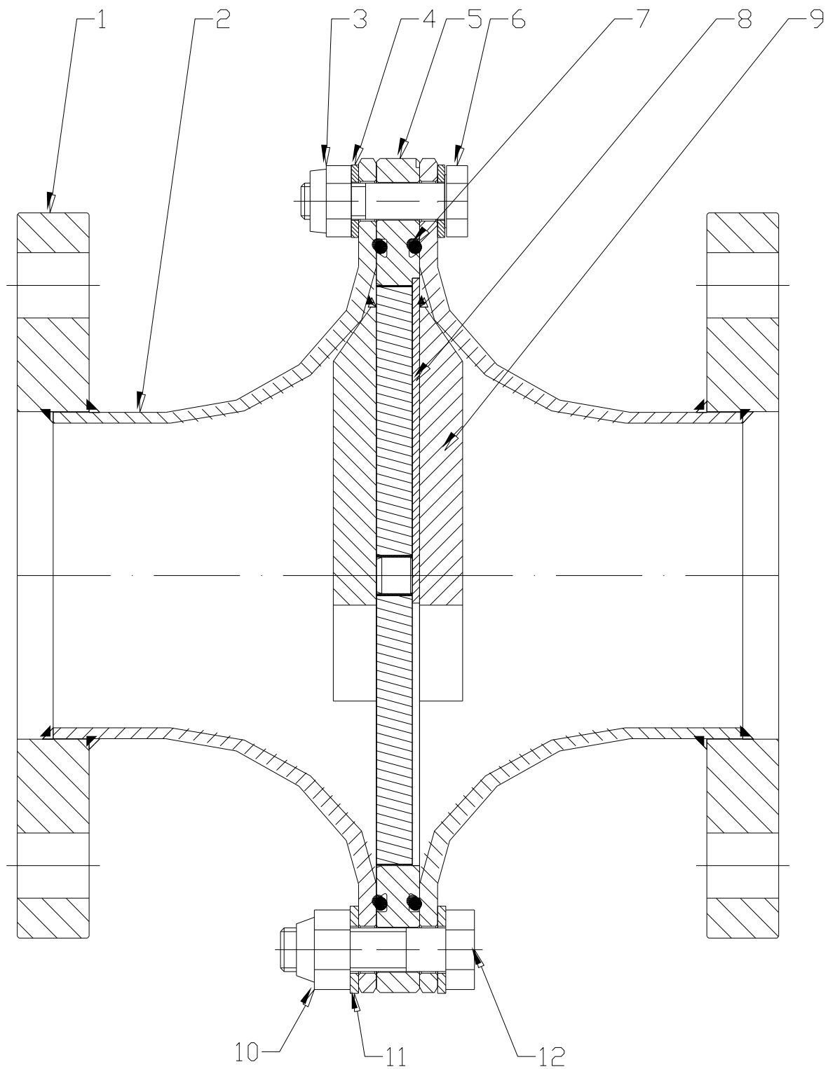
Fig. 1 Construction
