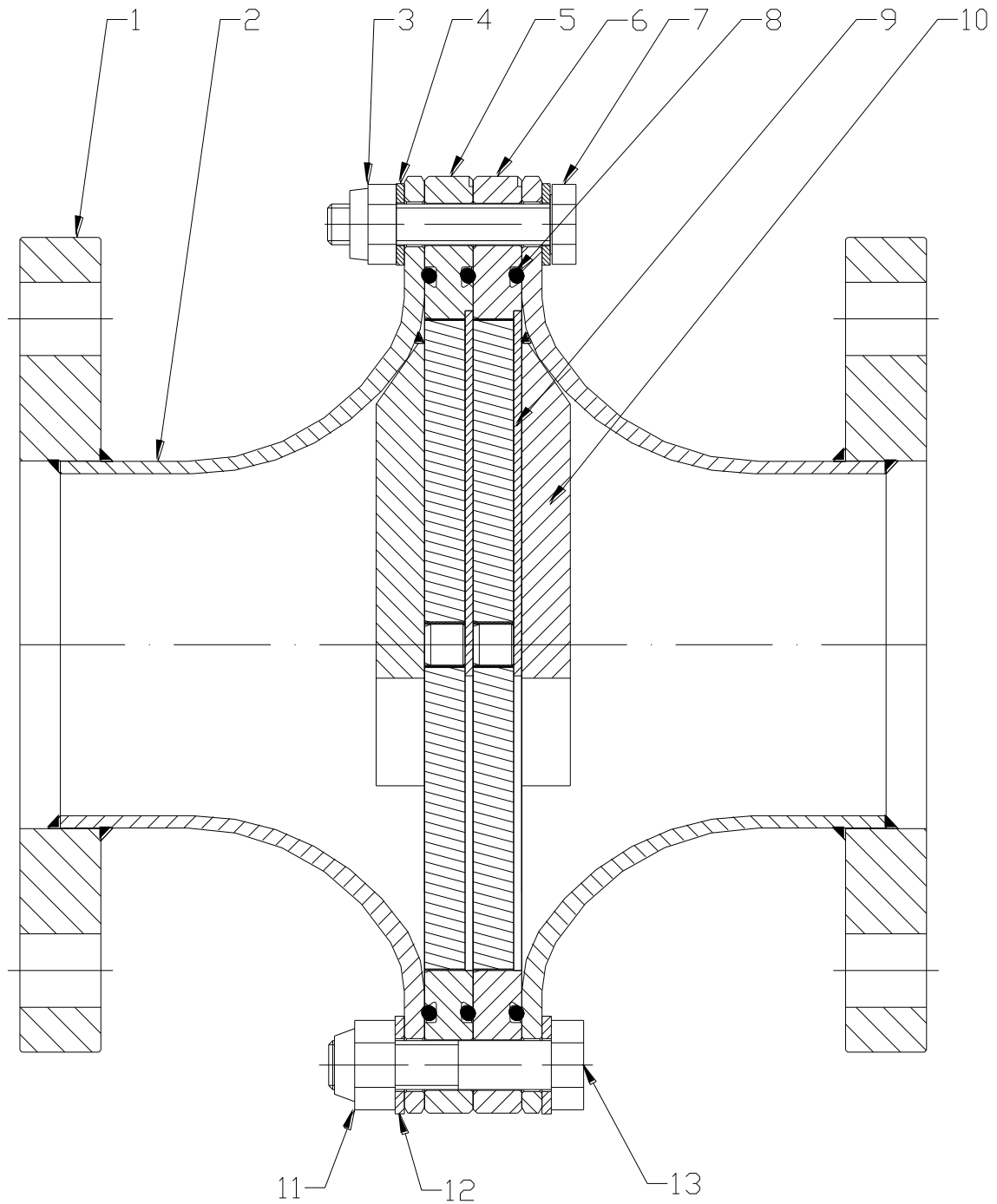
Fig. 1 Construction
