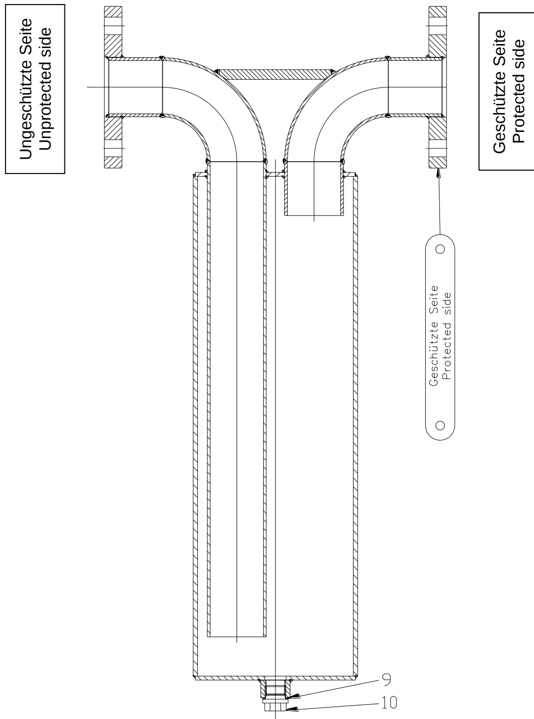
Fig. 1 Construction
