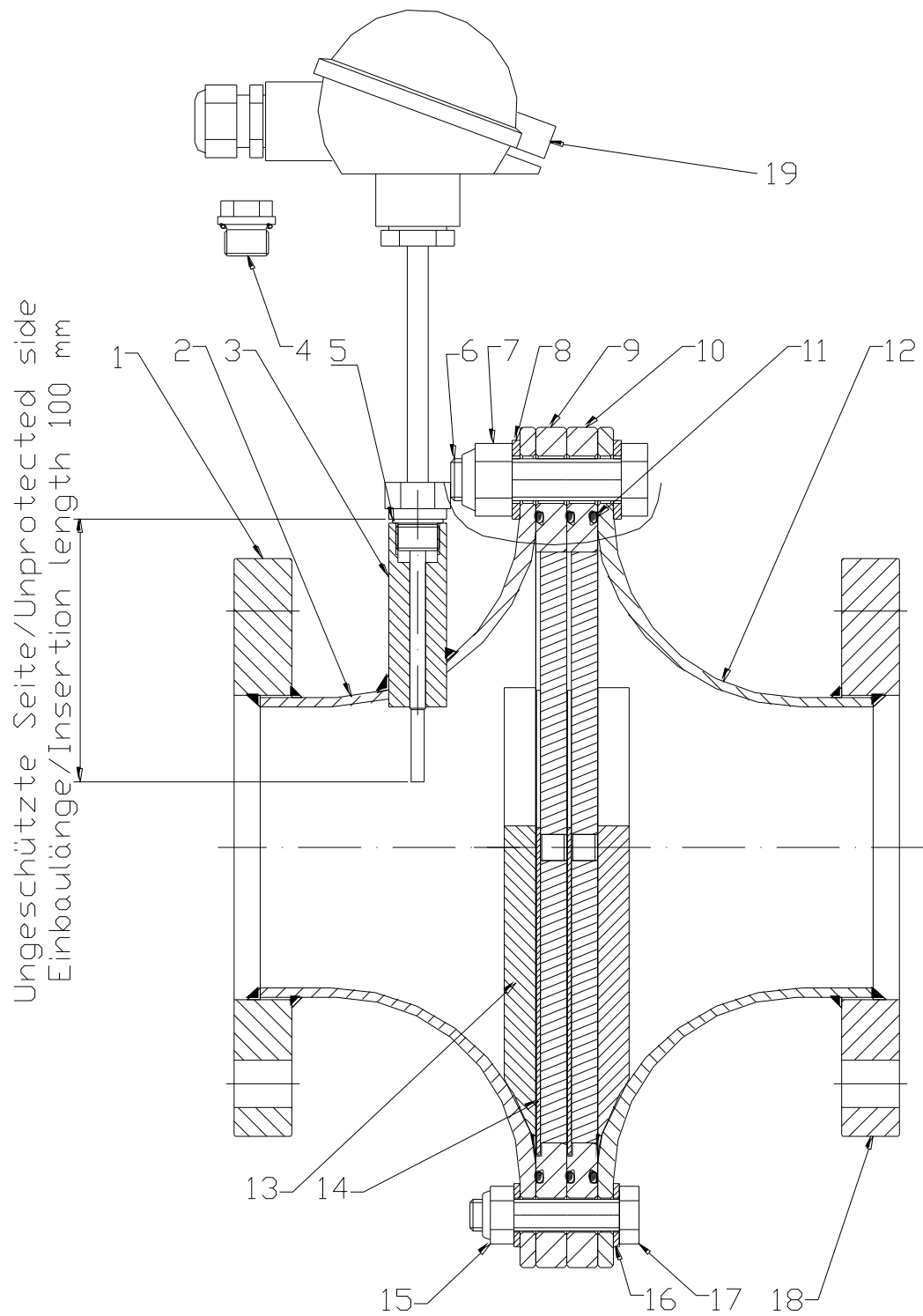
Fig. 1 Construction
