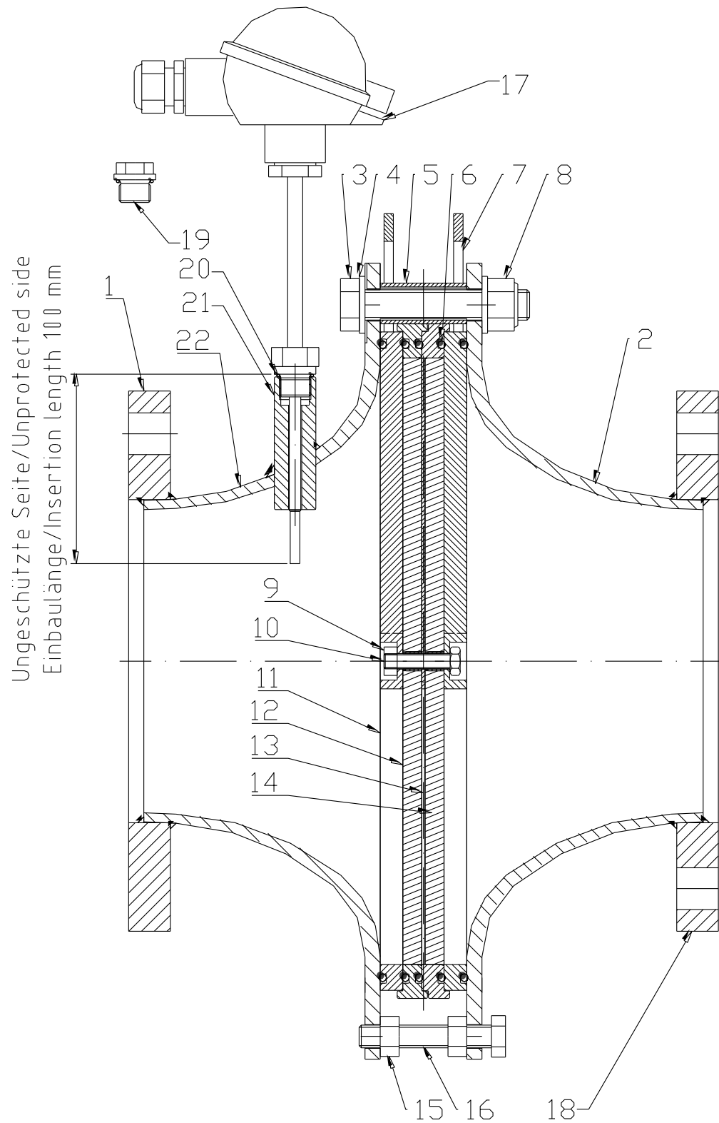
Fig. 1 Construction
